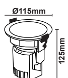
Dimension ( mm )
