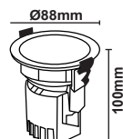
Dimension ( mm )
